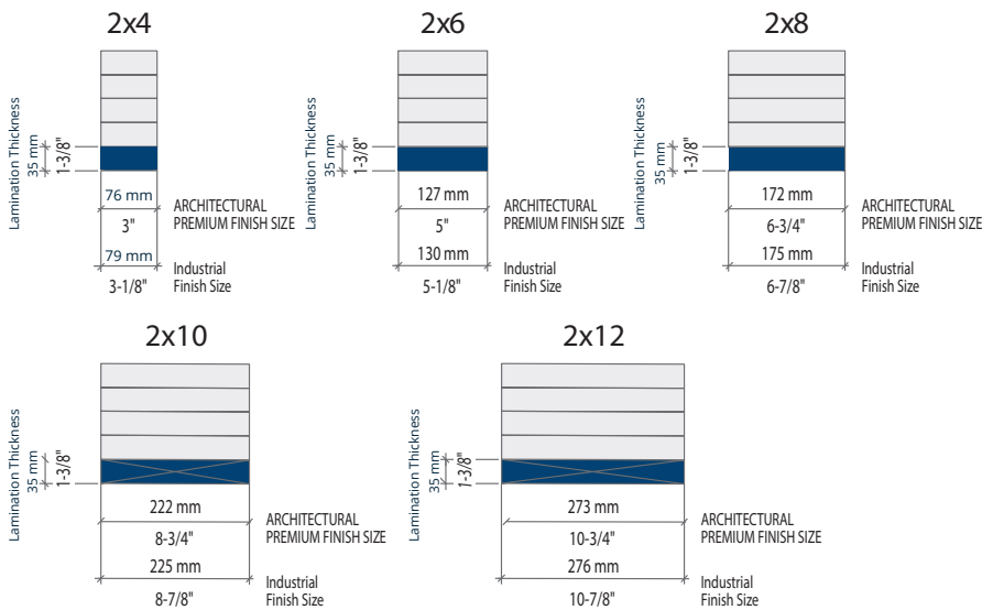
FIGURE 7: Single lamination beams
